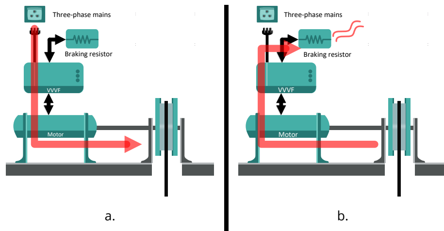
Fig. 8. Energy Exchange in a lift
