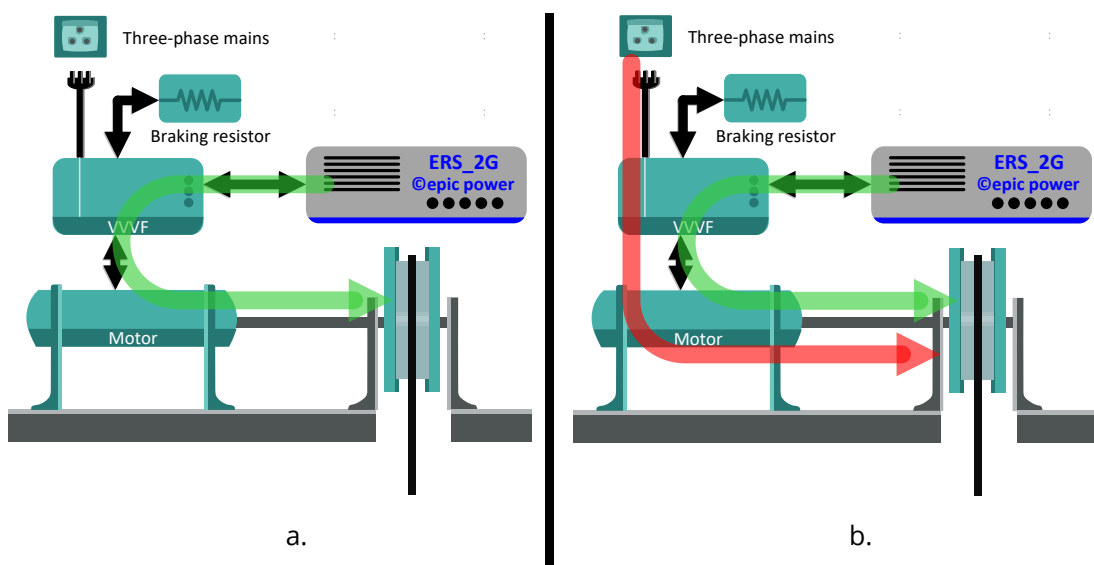
Fig. 11. Absorption energy flow
