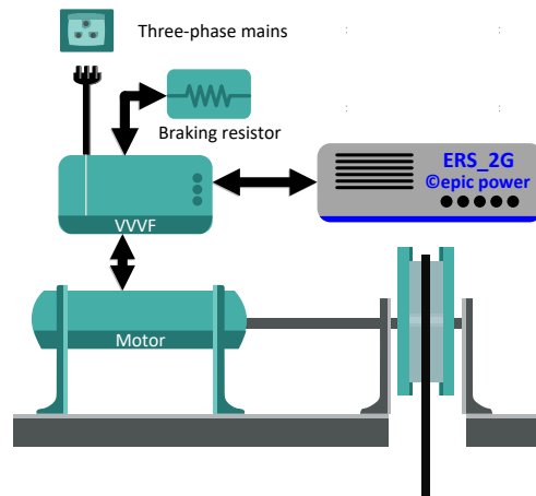
Fig. 9. ERS 2G connection to a lift traction system
