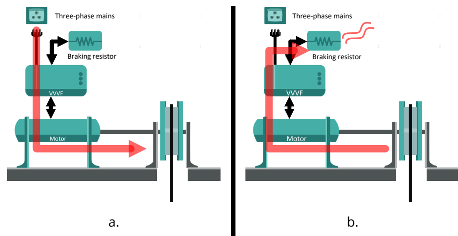
Fig. 8. Energy Exchange in a lift
