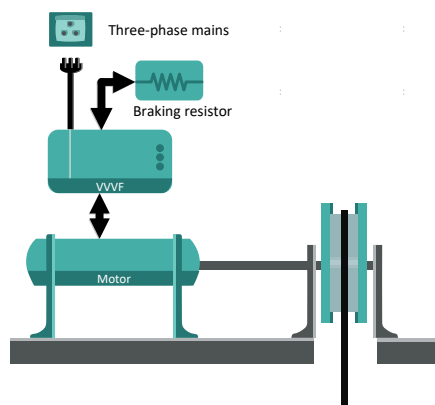
Fig. 7. Block diagram description of the electrical traction system of an elevator
