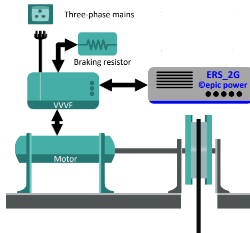
Fig. 9. ERS 2G connection to a lift traction system
