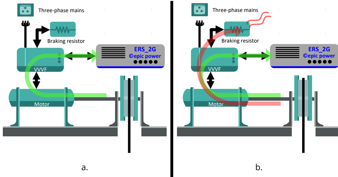
Fig. 10. Regenerative energy flows
