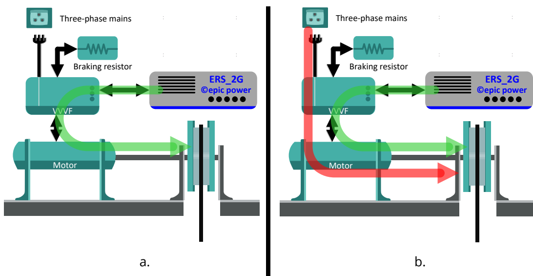
Fig. 11. Absorption energy flow
